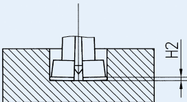
Sackloch-Tastkopf Blind bore probe
